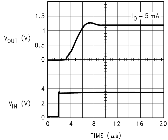
Enable Response
