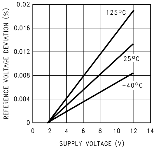
Line Regulation
