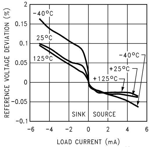
Load Regulation
