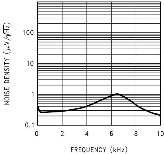
Noise Spectral Density (10Hz-10kHz)
