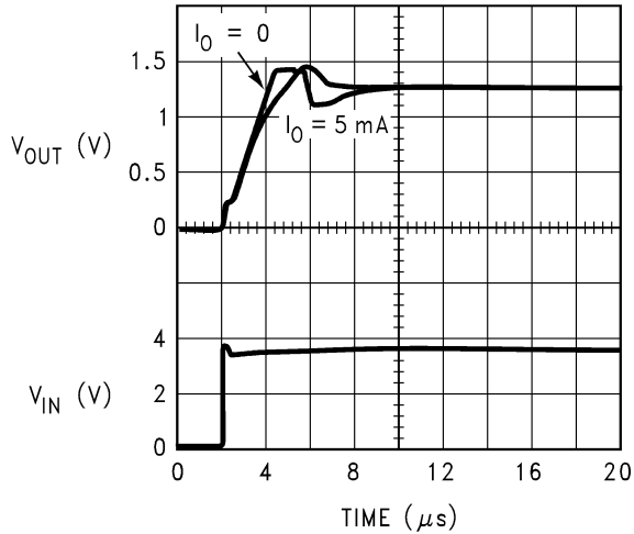
Start-Up Response
