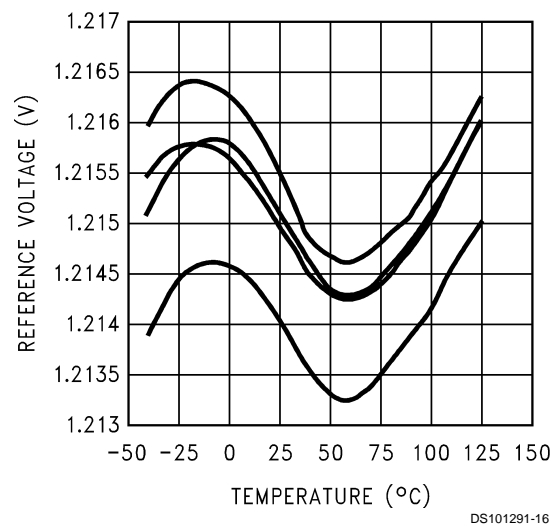
Typical Temperature Drift
