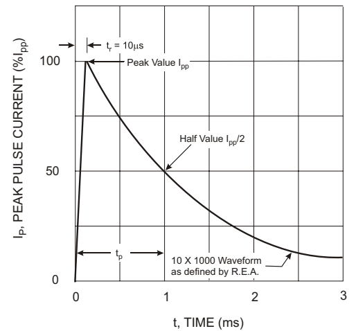
Fig. 4 Pulse Waveform
