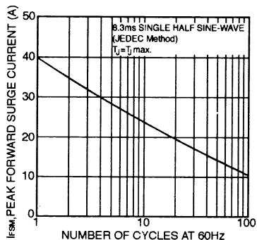
FIG. 5 – MAXIMUM NON-REPETITIVE PEAK FORWARD SURGE CURRENT
