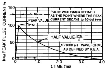
FIG. 3 – PULSE WAVEFORM
