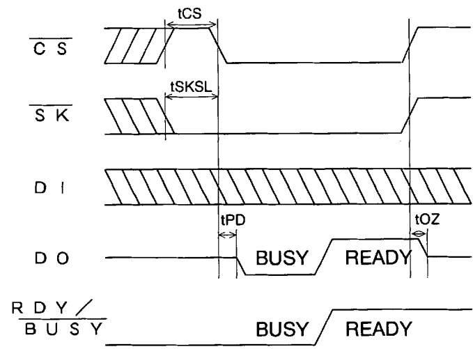
Ready / \overline{\text{BUSY}} Signal Output ( DO pin )
