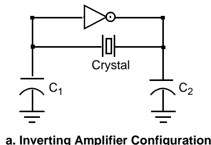
a. Inverting Amplifier Configuration
