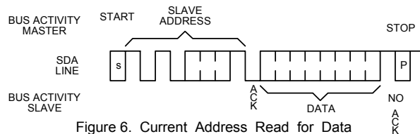
Figure 6. Current Address Read for Data
