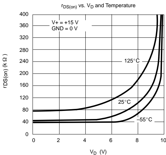
FIGURE 4. On-Resistance vs. Analog Signal Characteristics
