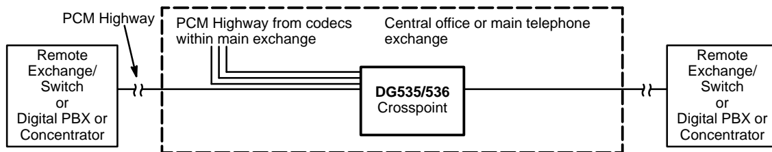
FIGURE 17. DG535/536 PCM Distribution Frame
