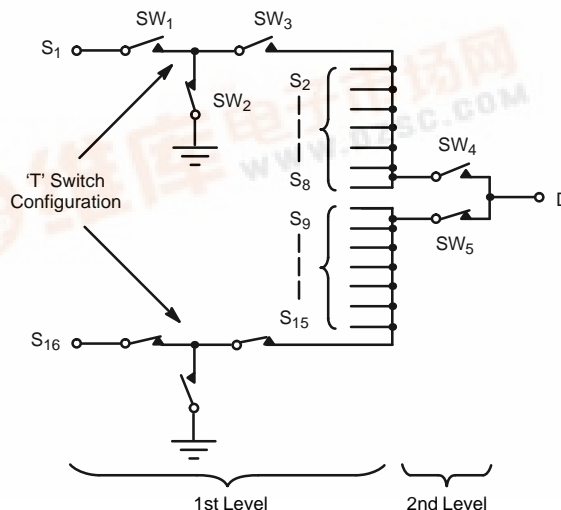
FIGURE 2. Switch Configuration
