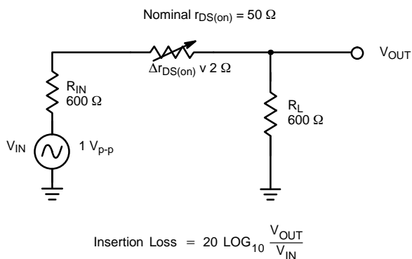
FIGURE 5. 600-Ω Audio System
