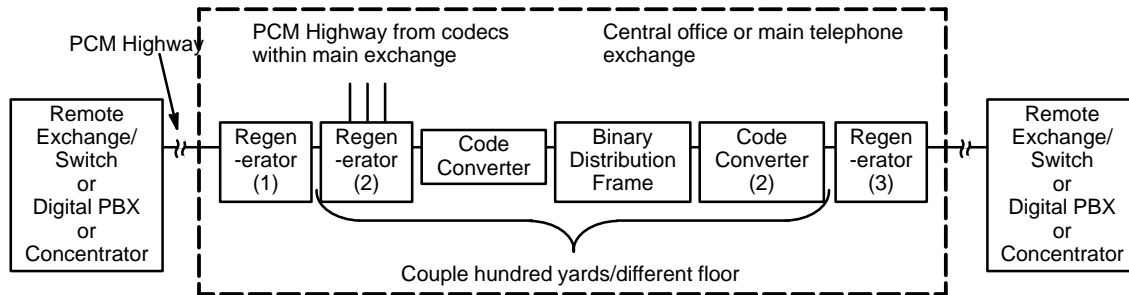
FIGURE 16. Binary PCM Routing Network
