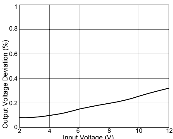
Line Regulation
