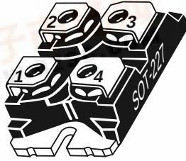
Parallel APT2X61D60J
