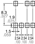
Recommended mounting pad (TOP VIEW)
