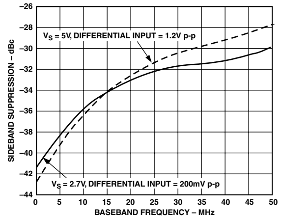
TPC 10. Sideband Suppression vs. F_{BB} . ( T_A = 25^\circ C , F_{LO} = 800 MHz, LO Level = -2 dBm, I and Q Inputs Driven in Quadrature)
