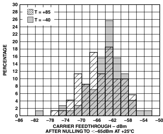
TPC 8. Carrier Feedthrough Distribution at Temperature Extremes. After Feedthrough Nulled to <-65 dBm at T_A = 25^\circ C . ( F_{LO} = 800 MHz, LO Level = -2 dBm)
