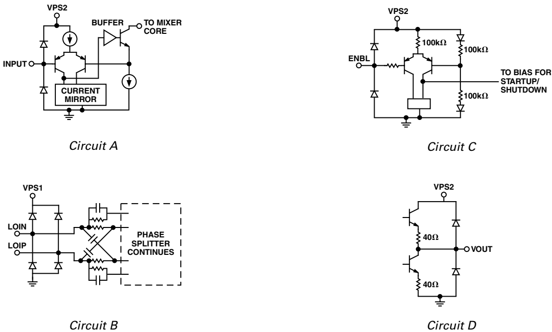
Figure 1. Equivalent Circuits
