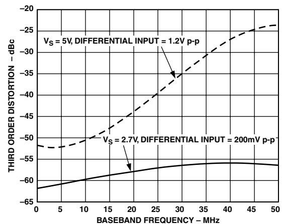
TPC 12. Third Order Distortion vs. F_{BB} . ( T_A = 25^\circ C , F_{LO} = 800 MHz, LO Level = -2 dBm, I and Q Inputs Driven in Quadrature)
