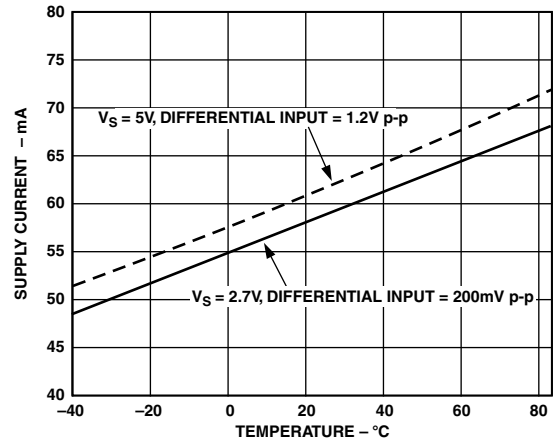
TPC 16. Power Supply Current vs. Temperature
