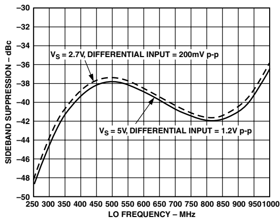
TPC 9. Sideband Suppression vs. F_{LO} . ( T_A = 25^\circ C , LO Level = -2 dBm, F_{BB} = 1 MHz, I and Q Inputs Driven in Quadrature)
