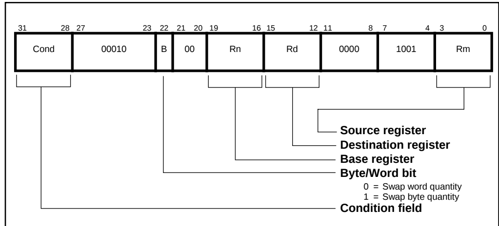
Figure 4-21: Swap instruction
