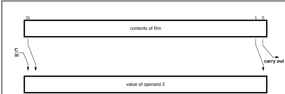
Figure 4-9: Rotate right extended
