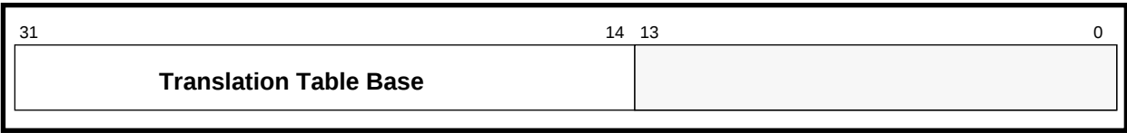
Figure 9-2: Translation table base register
