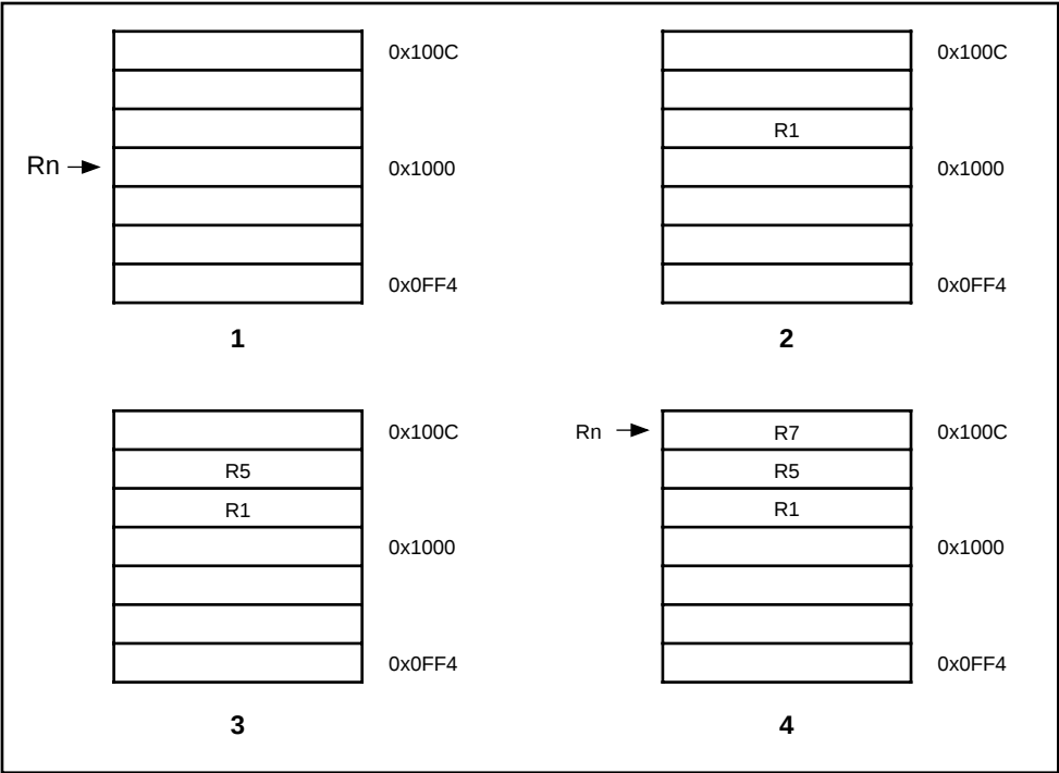
Figure 4-18: Pre-increment addressing
