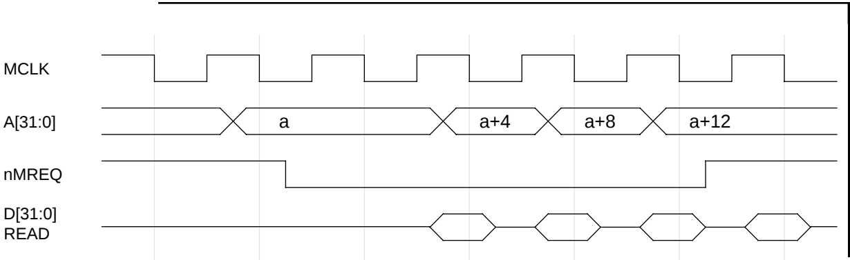
Figure 10-5: Linefetch
