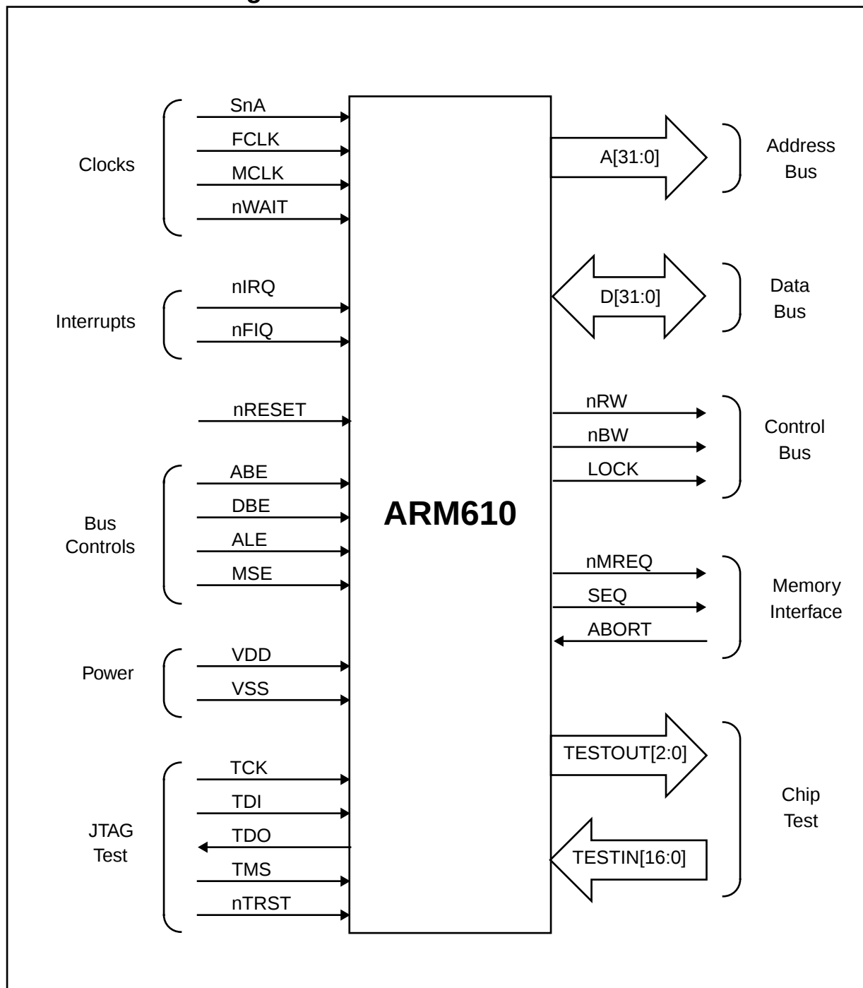
Figure 1-2: Functional diagram
