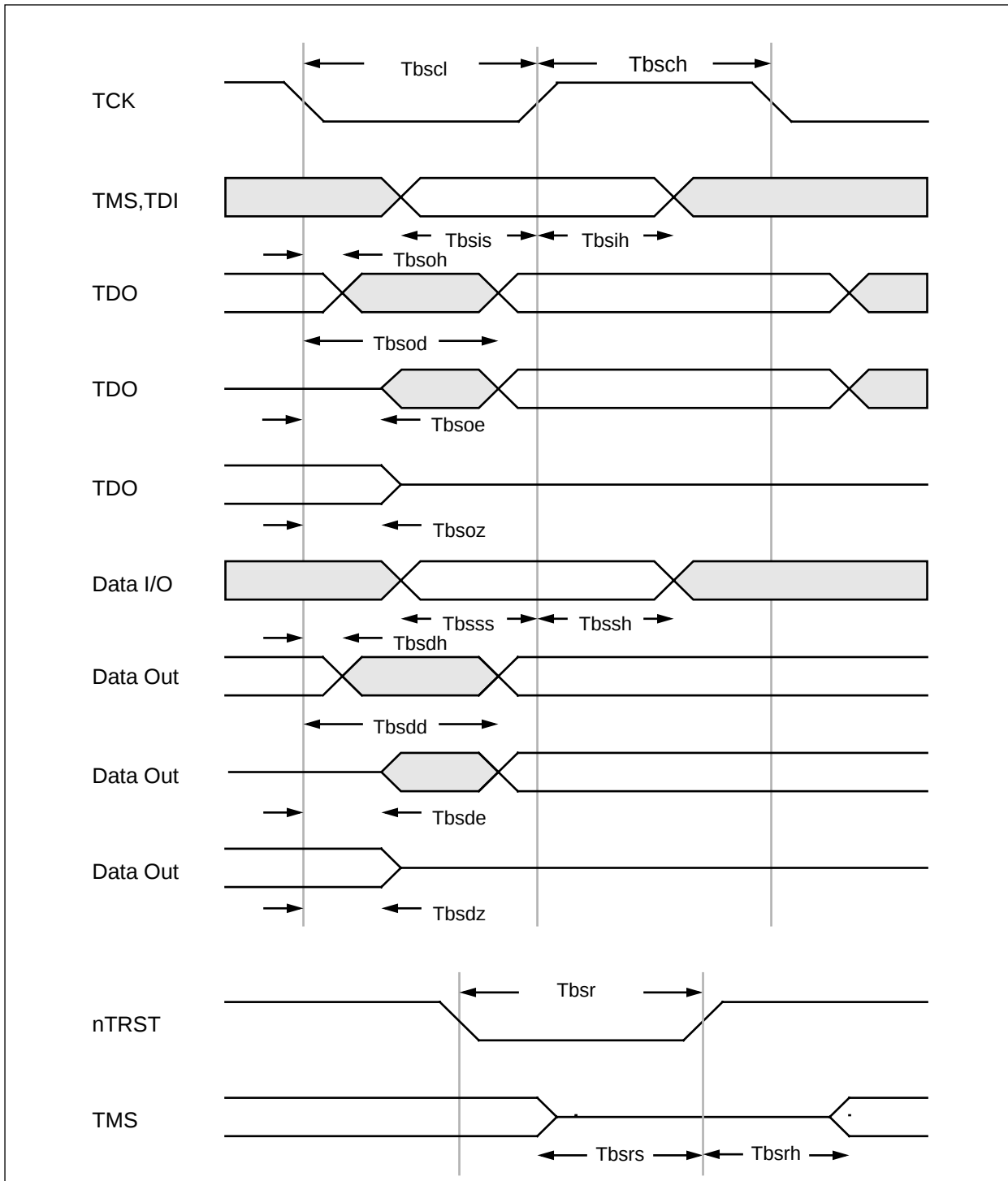
Figure 11-3: Boundary-scan timing
