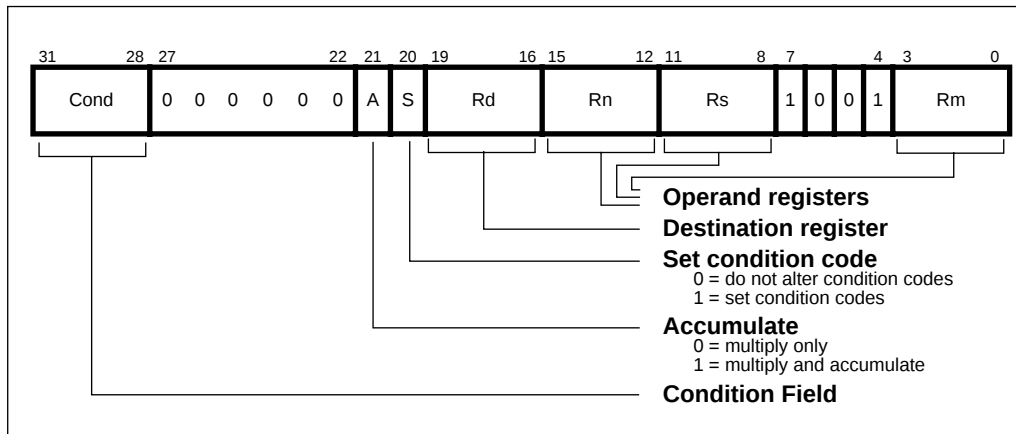
Figure 4-11: Multiply instructions
