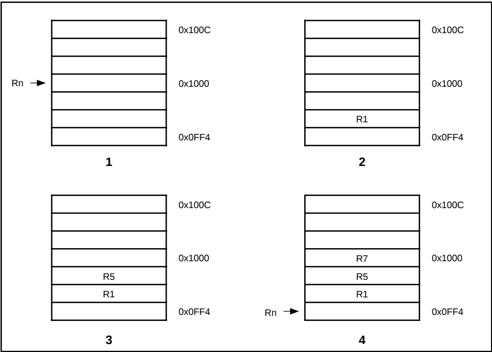
Figure 4-19: Post-decrement addressing
