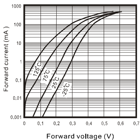
Fig. 1 - Forward characteristics
