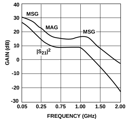
Figure 14. Insertion Power Gain, Maximum Available Gain, and Maximum Stable Gain vs. Frequency. V_{CE} = 6.0\text{ V} .
