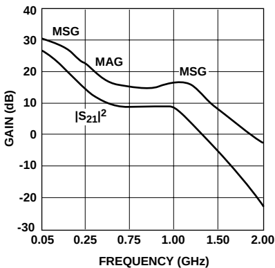
Figure 13. Insertion Power Gain, Maximum Available Gain, and Maximum Stable Gain vs. Frequency. V_{CE} = 4.8\text{ V} .
