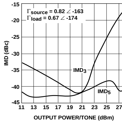
Figure 5. \text{IMD}_3 , \text{IMD}_5 vs. Output Power Per Tone.
