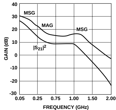
Figure 12. Insertion Power Gain, Maximum Available Gain, and Maximum Stable Gain vs. Frequency. V_{CE} = 3.6\text{ V} .
