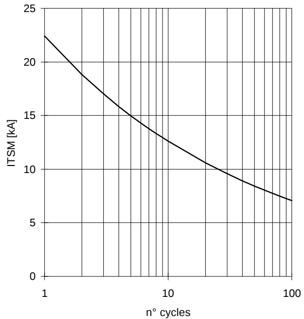
SURGE CHARACTERISTIC T_J = 125^\circ\text{C}
