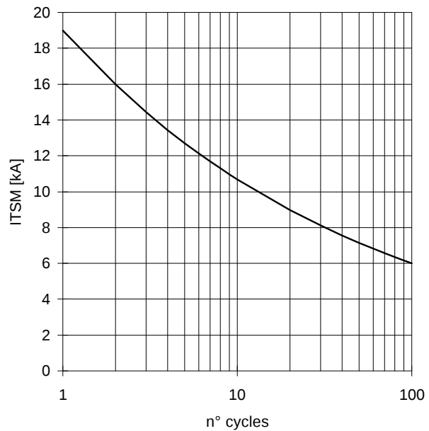
SURGE CHARACTERISTIC T_J = 125^\circ\text{C}
