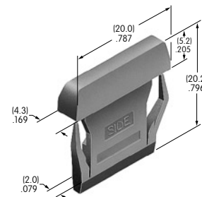
AT497 End Barrier Polyamide Color: A Series: LB
