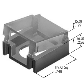
AT494 Protective Guard Polycarbonate & polyamide Series: KB
