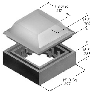
AT499 Protective Guard for Square Polycarbonate & polyamide Series: LB
