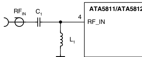
Figure 7. Input Matching to 50 \Omega
