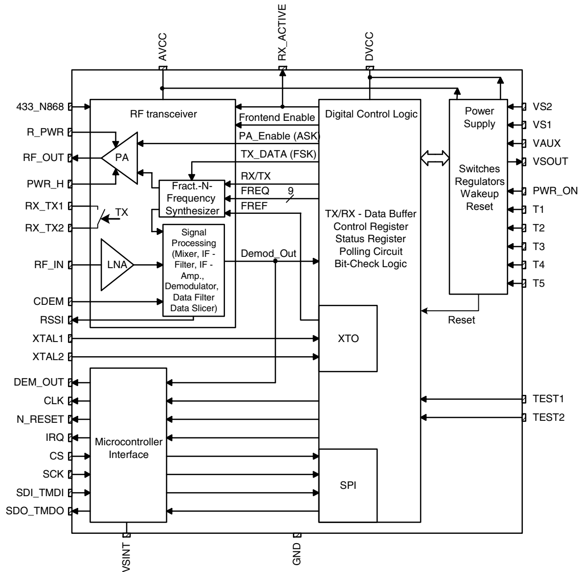
Figure 3. Block Diagram
