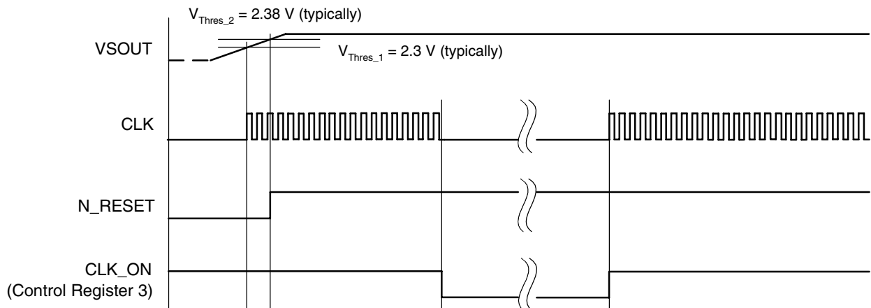
Figure 20. Clock Timing
