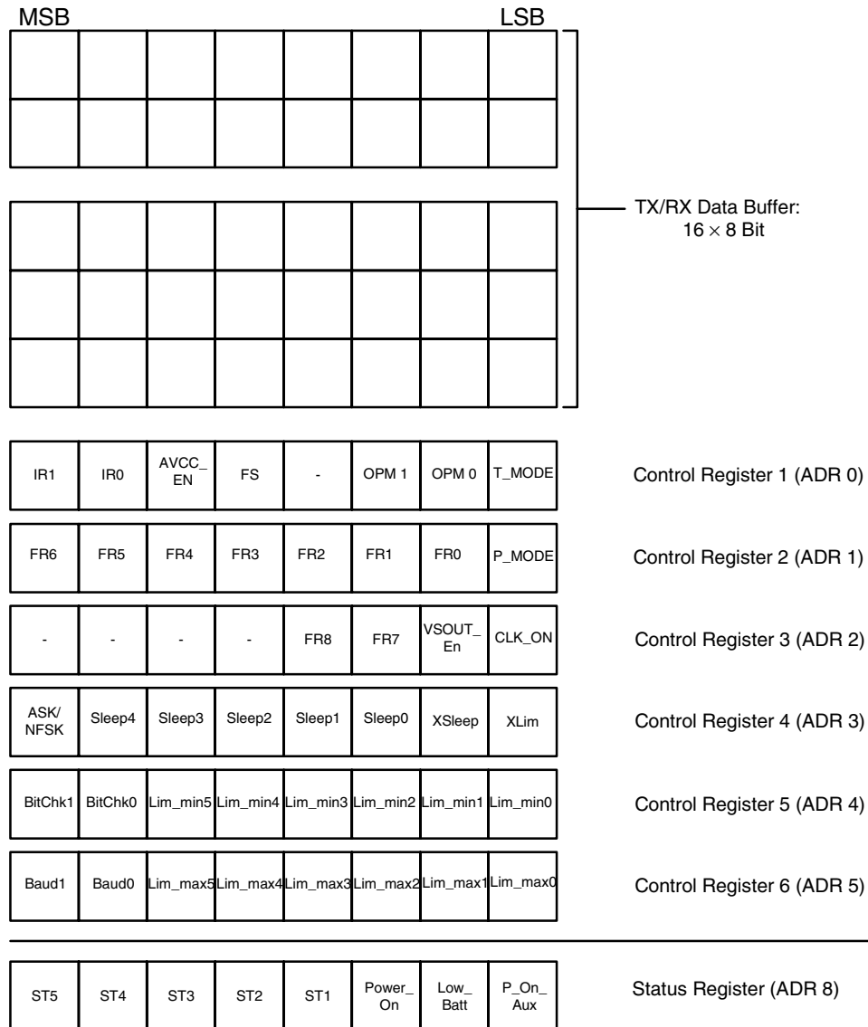
Figure 27. Register Structure
