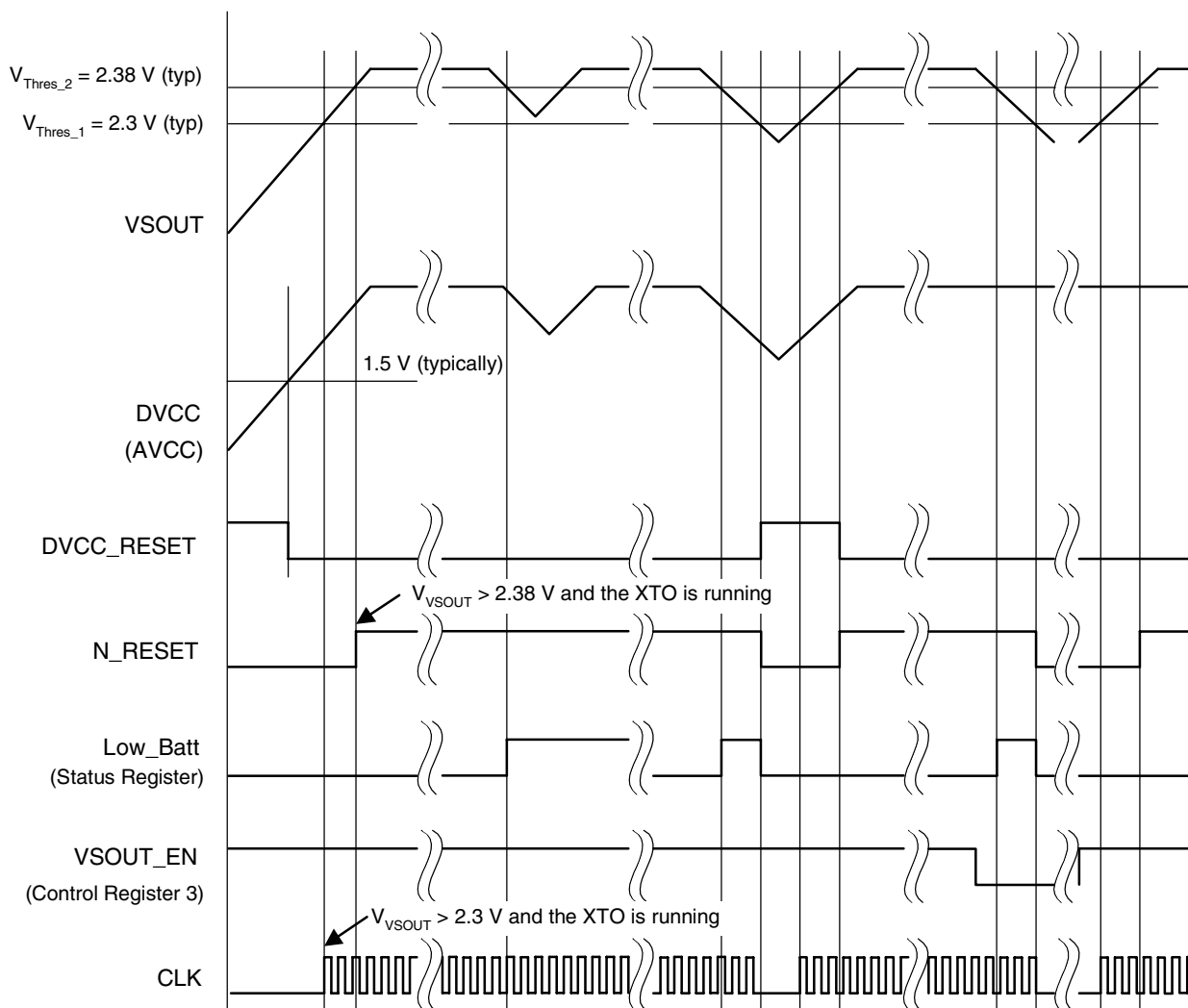
Figure 23. Reset Timing
