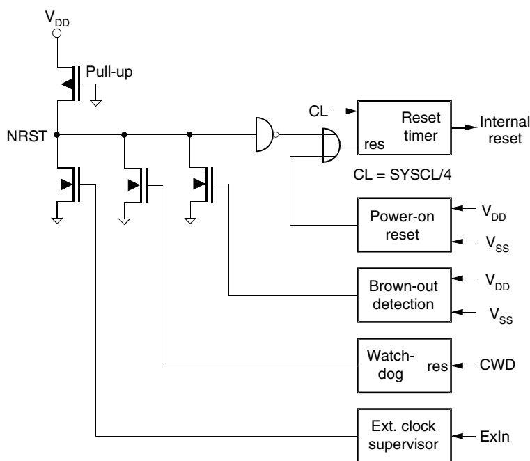
Figure 9. Reset Configuration
