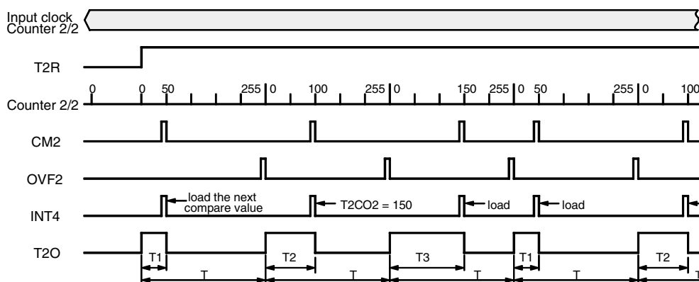
Figure 41. PWM Modulation
