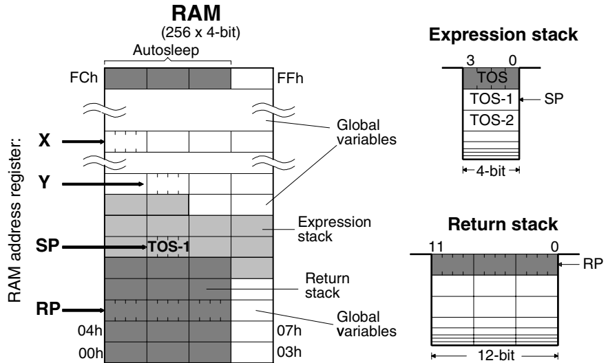
Figure 5. RAM Map
