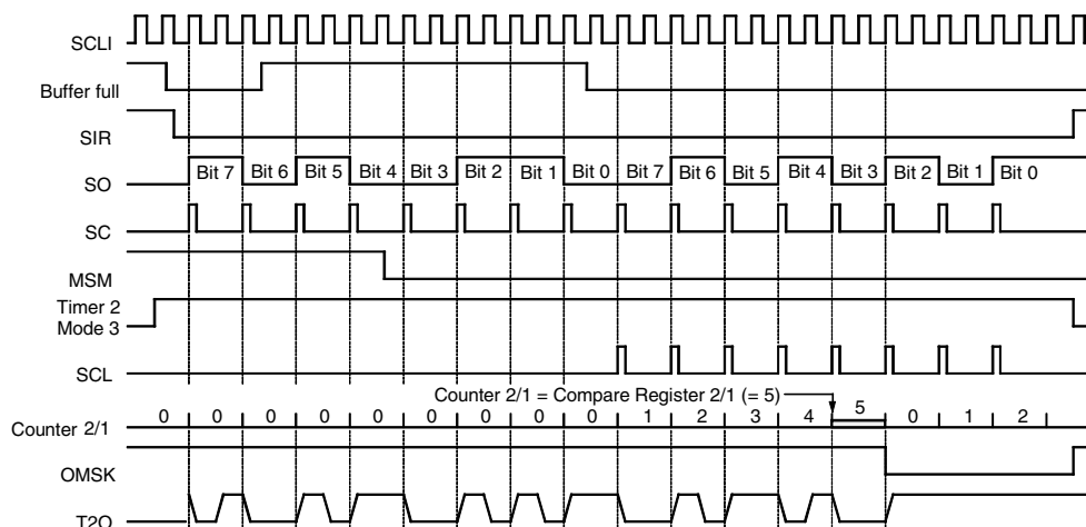
Figure 58. Bi-phase Modulation 2
