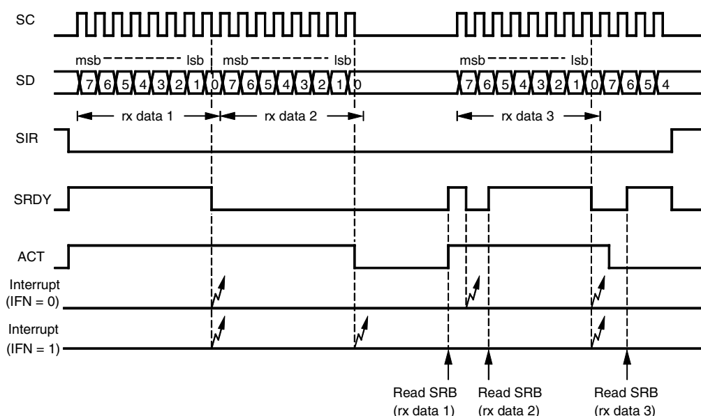
Figure 46. Example of 8-bit Synchronous Receive Operation
