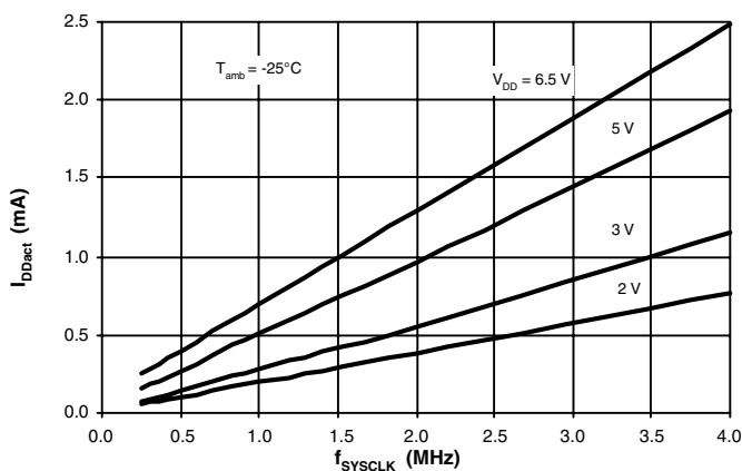
Figure 64. Power-down Supply Current versus Frequency
