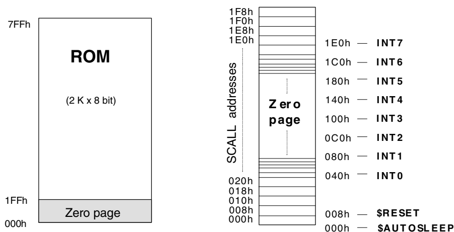
Figure 4. ROM Map
