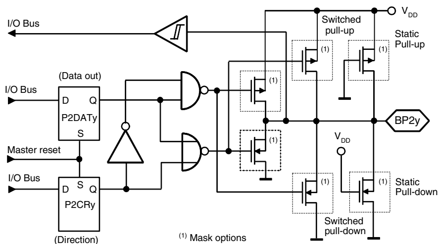
Figure 22. Bi-directional Port 2
