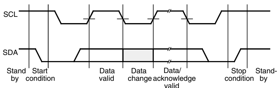
Figure 61. MCL Protocol
