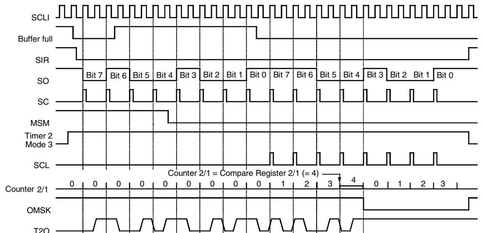
Figure 57. Manchester Modulation 2
