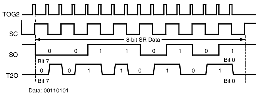
Figure 40. Manchester Modulation
