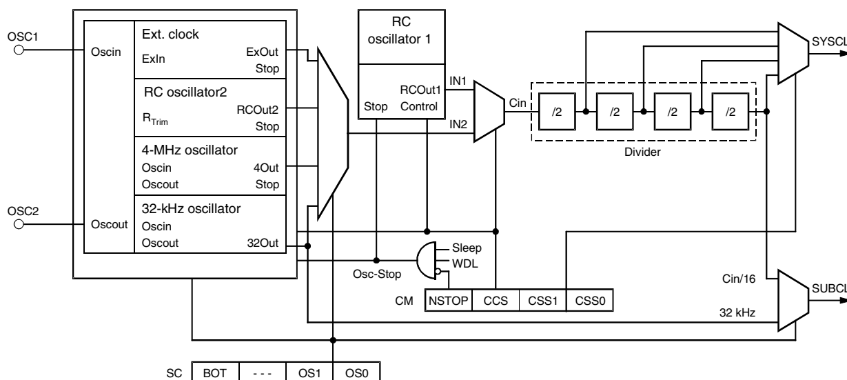
Figure 14. Clock Module
