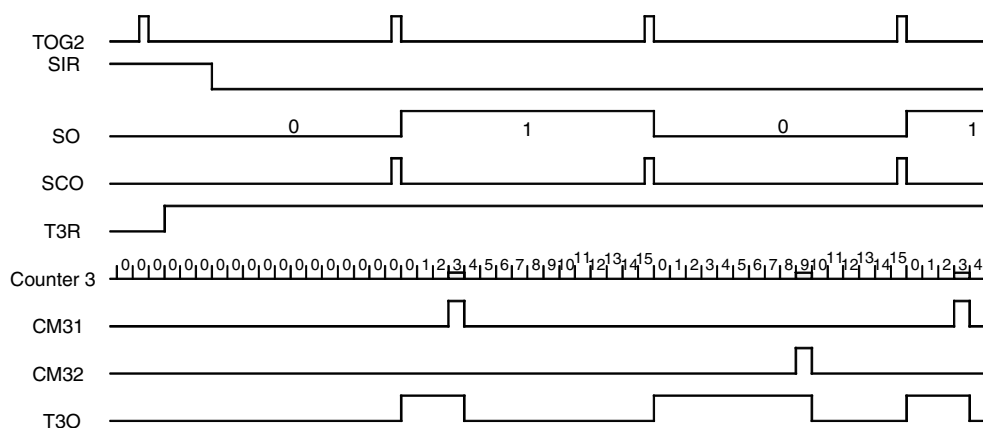
Figure 76. Pulse-width Modulation
