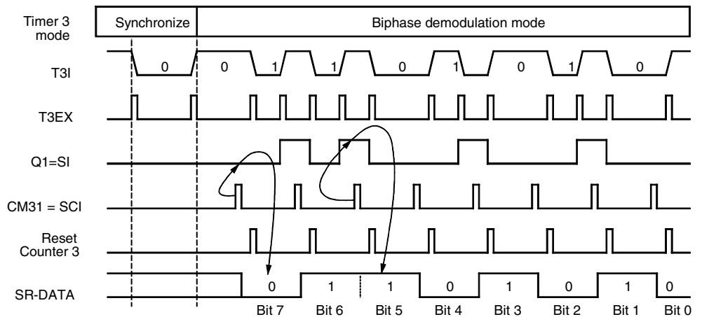
Figure 78. Bi-phase Demodulation
