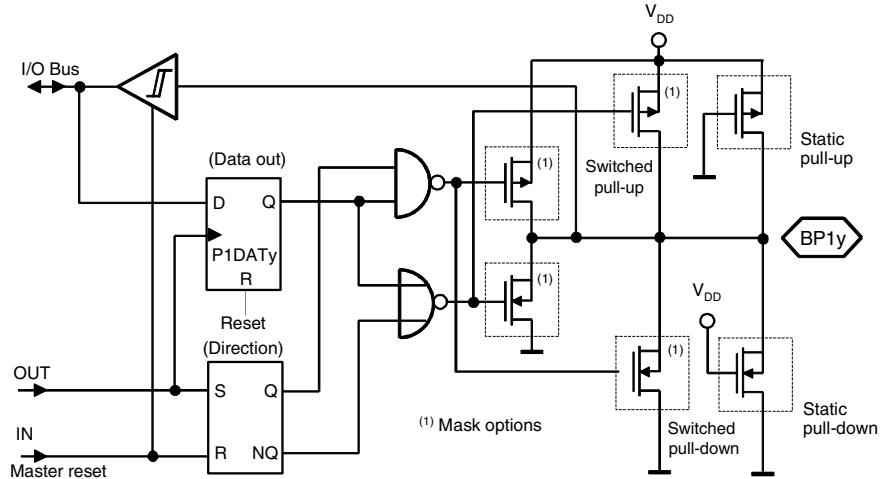
Figure 22. Bidirectional Port 1
