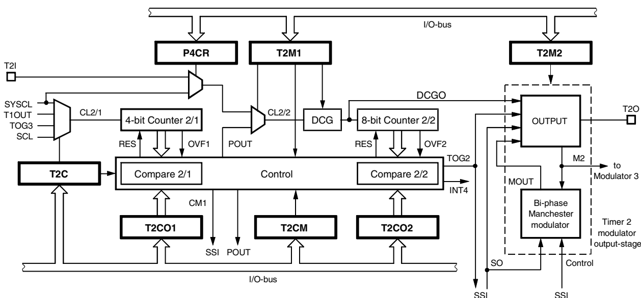
Figure 30. Timer 2
