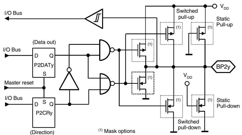
Figure 23. Bidirectional Port 2
