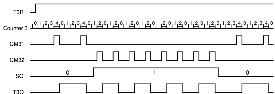
Figure 75. FSK Modulation 1
