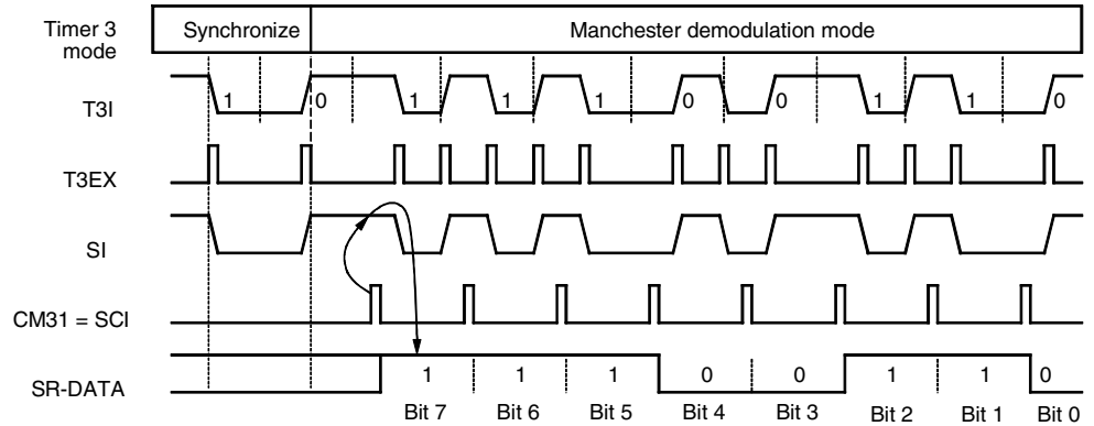
Figure 77. Manchester Demodulation
