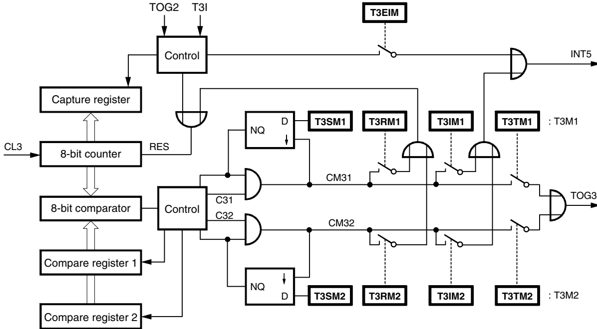
Figure 45. Counter 3 Stage
