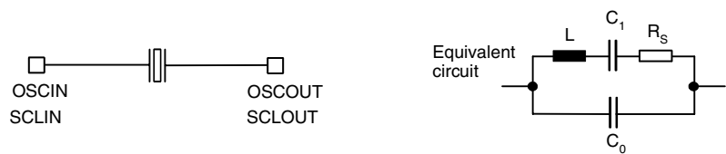
Figure 89. Crystal Equivalent Circuit
