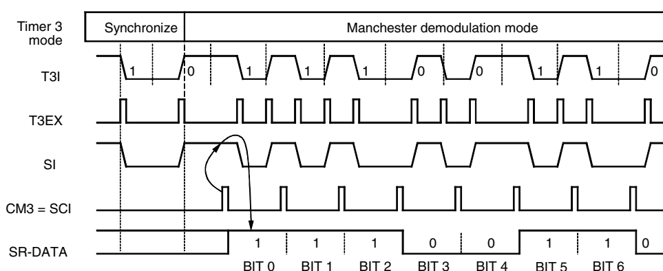
Figure 53. Timer 3 – Manchester Demodulation
