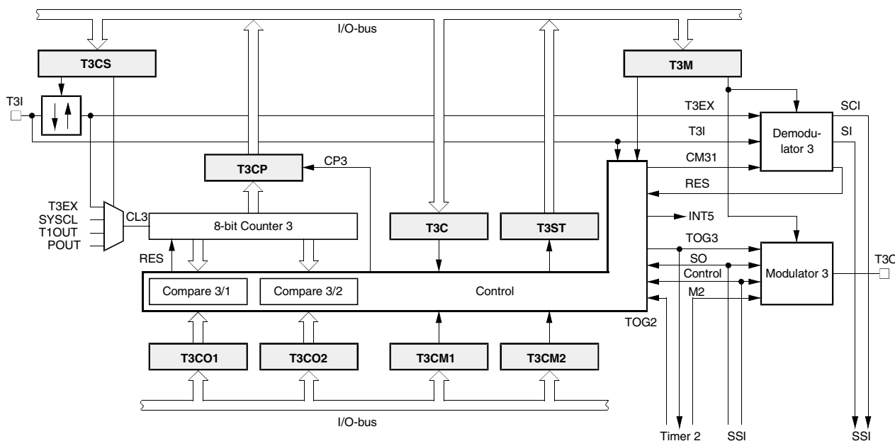
Figure 44. Timer 3
