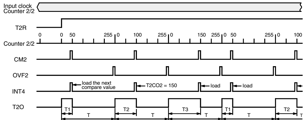
Figure 42. PWM Modulation
