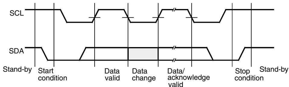
Figure 88. MCL Protocol
