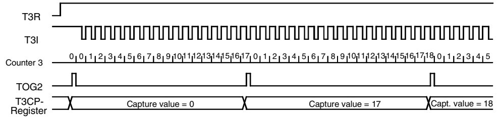
Figure 80. Frequency Measurement
