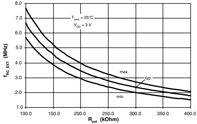
Figure 101. External RC Frequency versus R_{ext}
