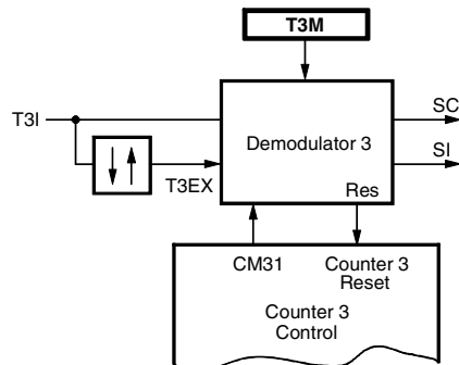
Figure 57. Timer 3 – Demodulator 3
