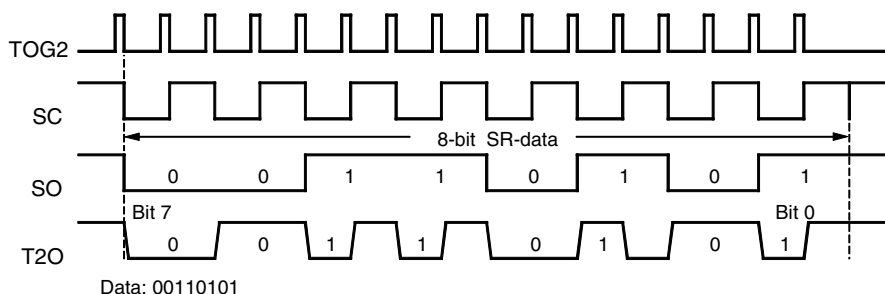
Figure 70. Bi-phase Modulation 1
