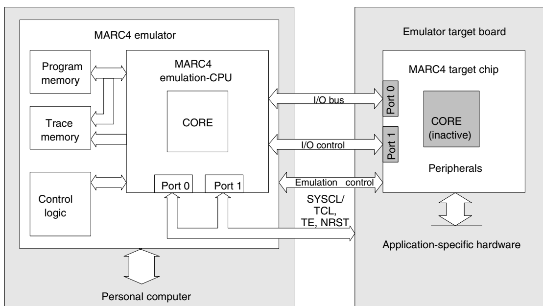
Figure 110. MARC4 Emulation
