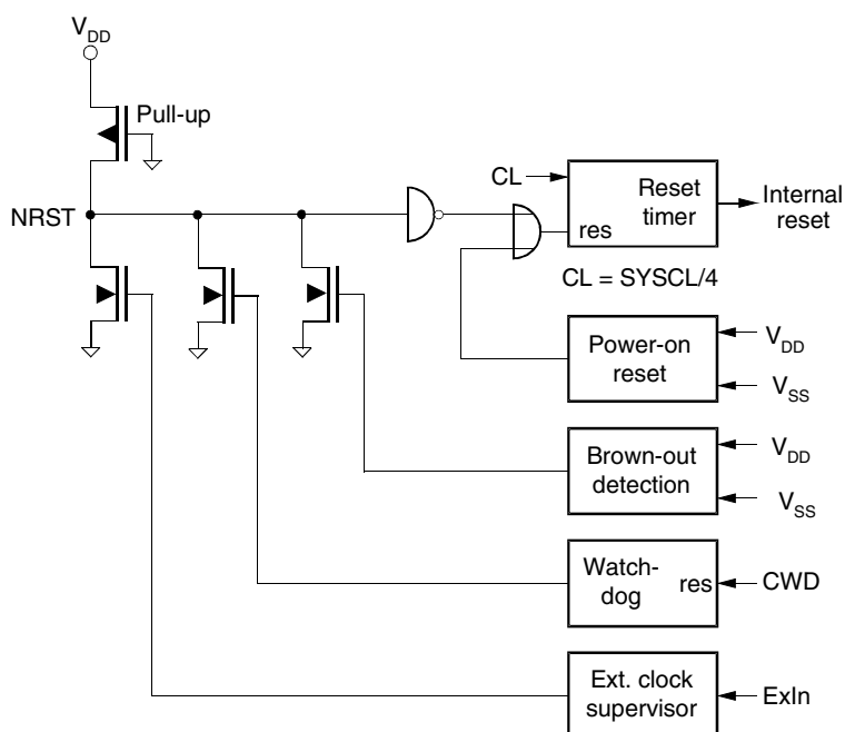
Figure 9. Reset Configuration
