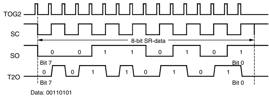
Figure 71. Manchester Modulation 1
