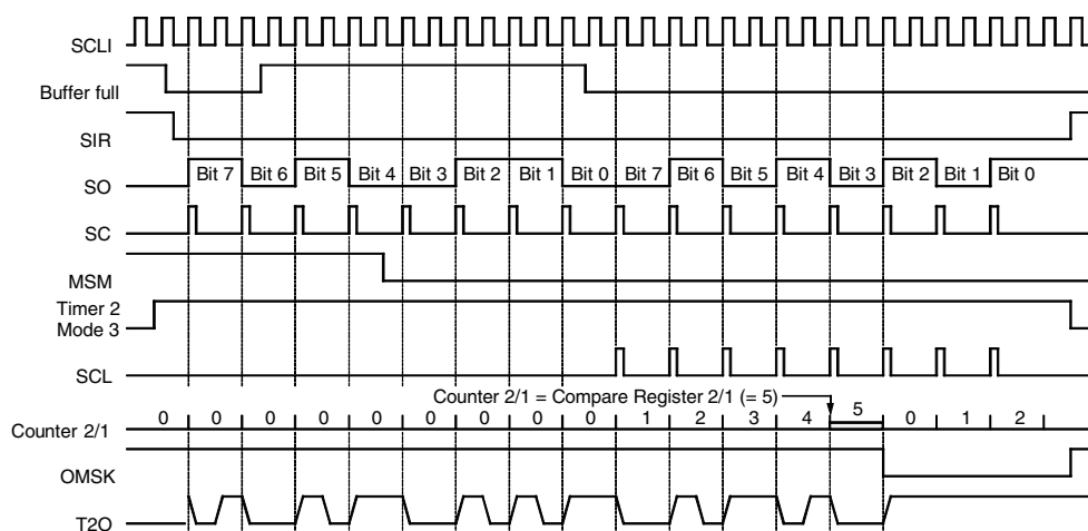
Figure 73. Bi-phase Modulation 2
