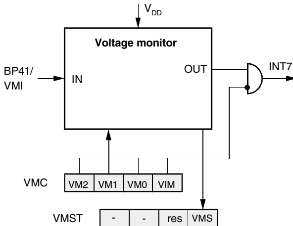
Figure 11. Voltage Monitor
