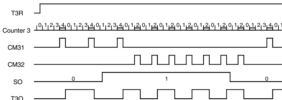
Figure 85. FSK Modulation
