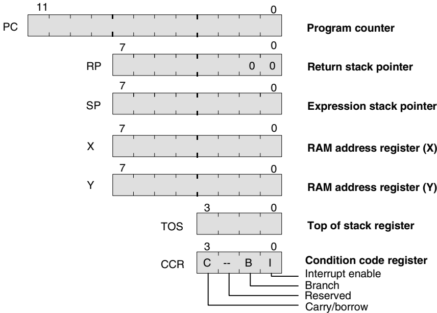
Figure 6. Programming Model
