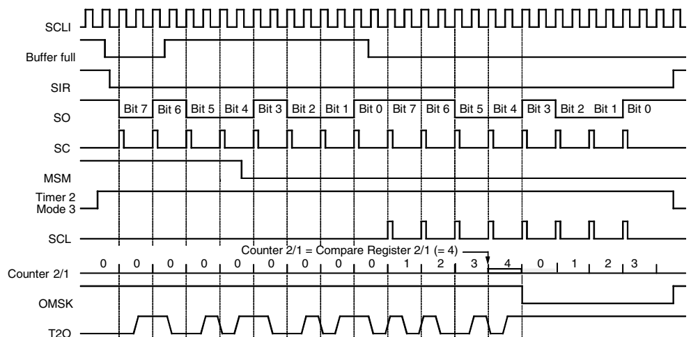
Figure 72. Manchester Modulation 2
