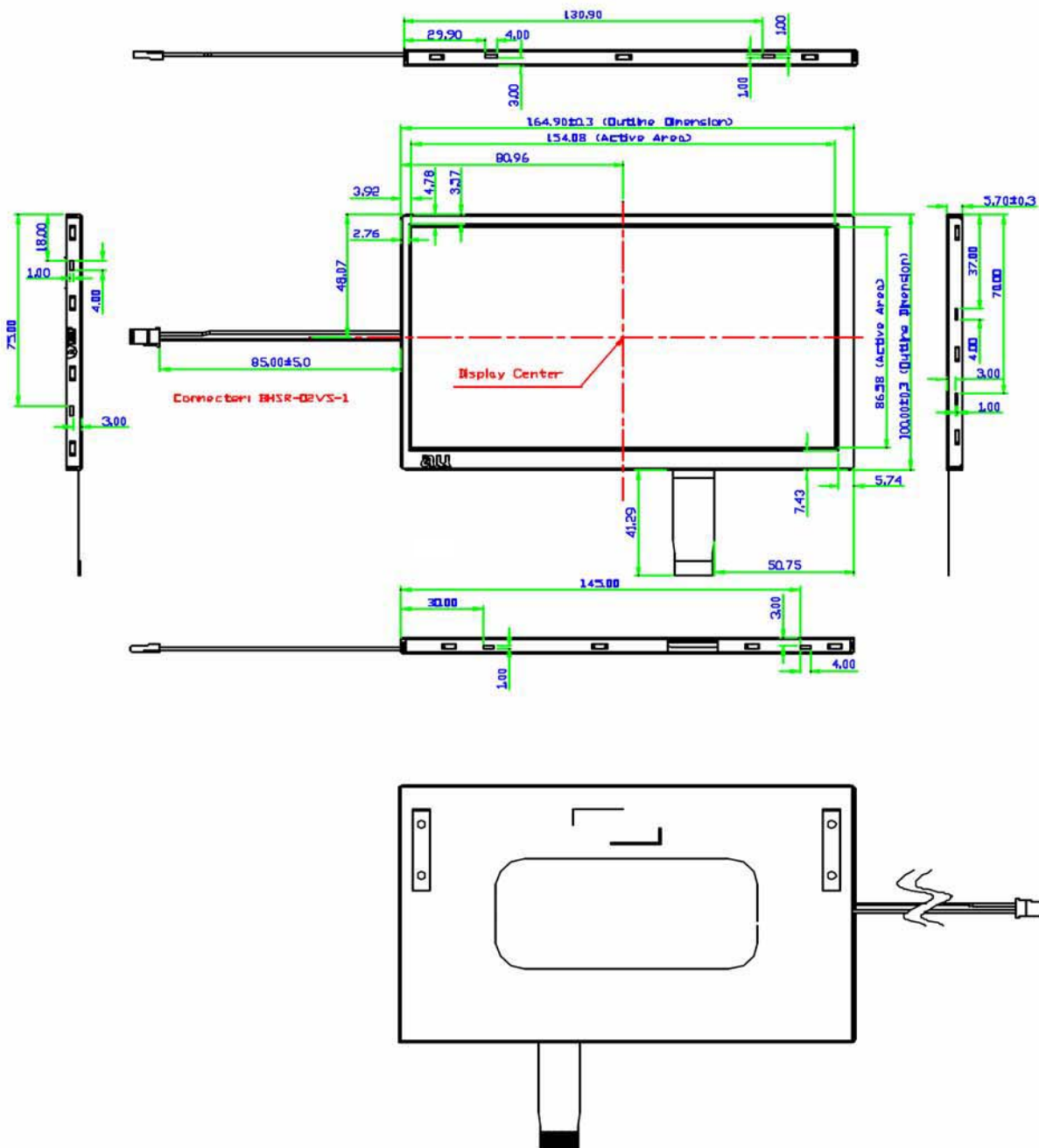
Fig.1- Outline dimension of TFT-LCD module
