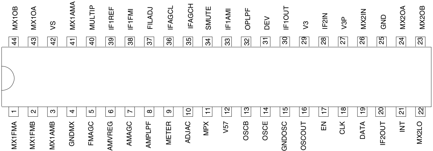
Figure 2. Pinning SSO44
