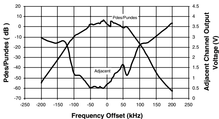
Figure 18. Selectivity
