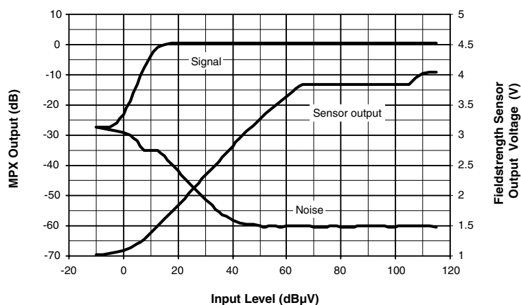
Figure 17. FM Input Level Sweep
