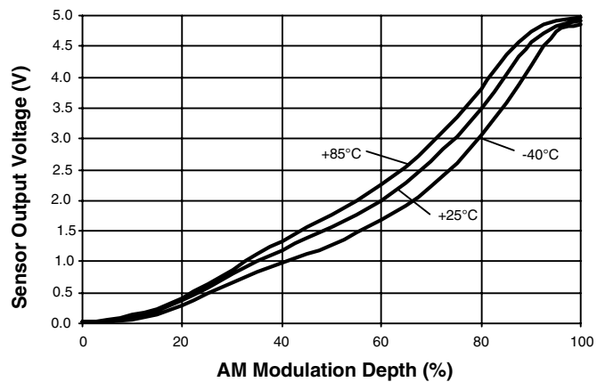
Figure 13. Multipath Sensor
