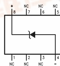
SO Package
