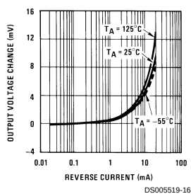
Reverse Characteristics
