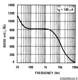
Noise Voltage
