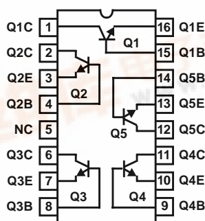
HS1-6254RH (CERDIP) GDIP1-T16 OR HS1-6254RH (SBDIP) CDIP2-T16 TOP VIEW
