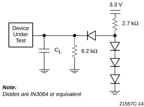
Figure 11. Test Setup
