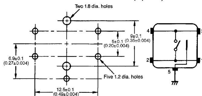
Terminal arrangement/ Internal connection (top view)
