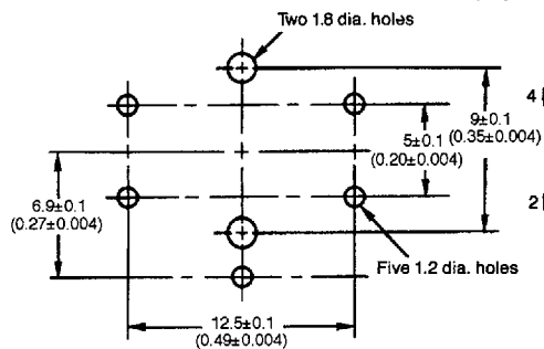
Terminal arrangement/ Internal connection (top view)
