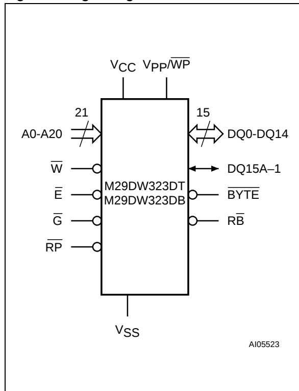
Figure 2. Logic Diagram
