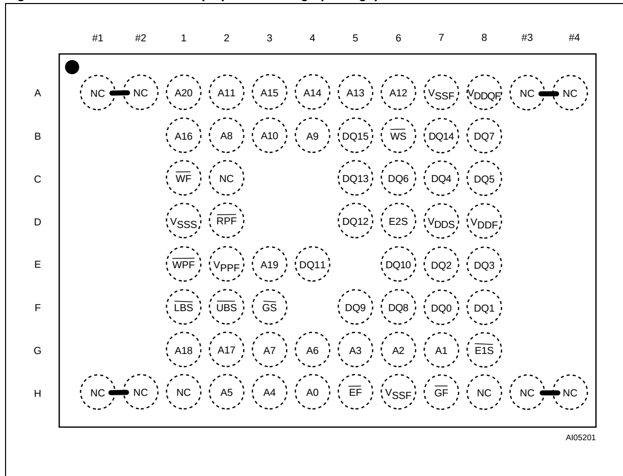
Figure 3. LFBGA Connections (Top view through package)
