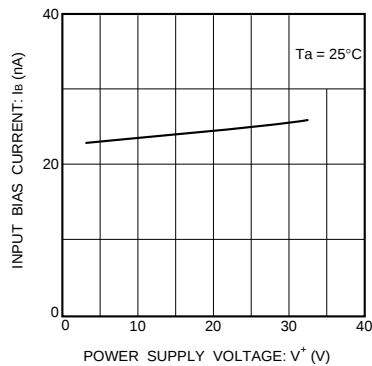
Fig. 3 Input bias current vs. power supply voltage
