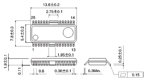
HSOP-25
