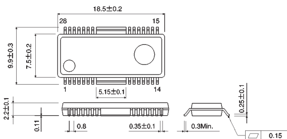
HSOP-M28
