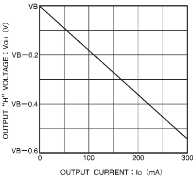
Fig.7 Output high level voltage vs. output current
