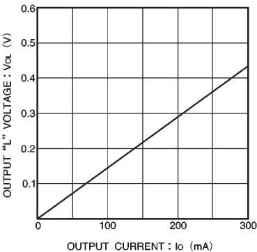
Fig.8 Output low level voltage vs. output current
