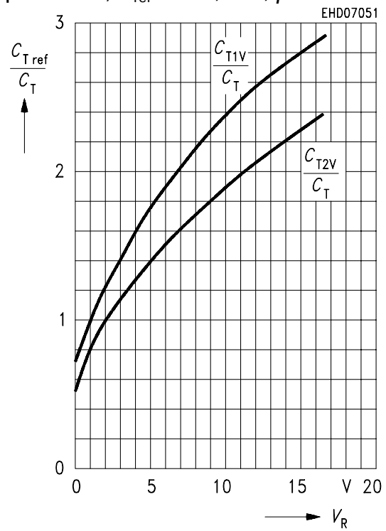
Capacitance ratio C_T/C_{Tref} = f(V_R) per diode; V_{ref} = 1 V, 2 V, f = 1 MHz
