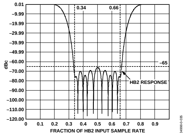
Figure 35. HB2 Filter Response to the Input Rate of the Filter
