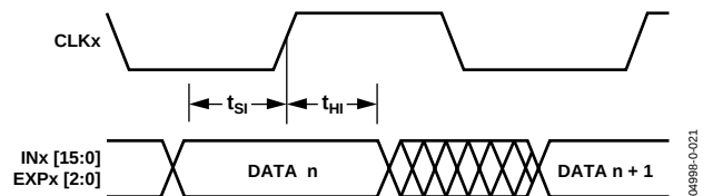
Figure 21. Input Data Timing Requirements (Rising Edge of Clock, x = A, B, C, or D for Four Input Ports)
