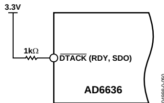
Figure 50. \overline{\text{DTACK}} , SDO Pull-Up Resistor Circuit
