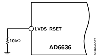
Figure 52. LVDS_RSET Circuit for LVDS Calibration
