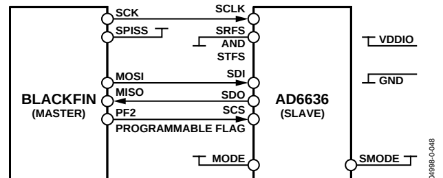
Figure 48. SPI Mode Serial Port Connections to Blackfin DSP
