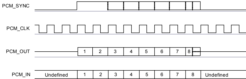
Figure 10.21: Long Frame Sync (Shown with 8-bit Companded Sample)
