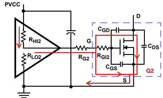
FIGURE 4. TYPICAL LOWER-GATE DRIVE TURN-ON PATH
