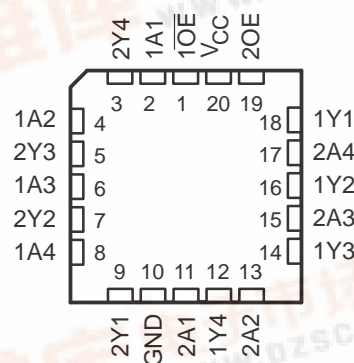
SN54BCT241 . . . FK PACKAGE (TOP VIEW)
