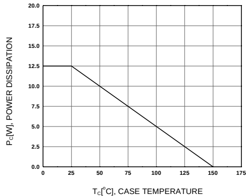
Figure 5. Power Derating
