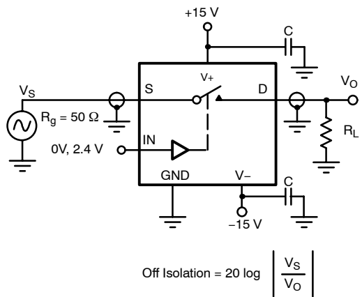
FIGURE 5. Off Isolation
