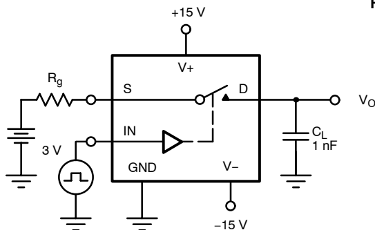
FIGURE 2. Switching Time
