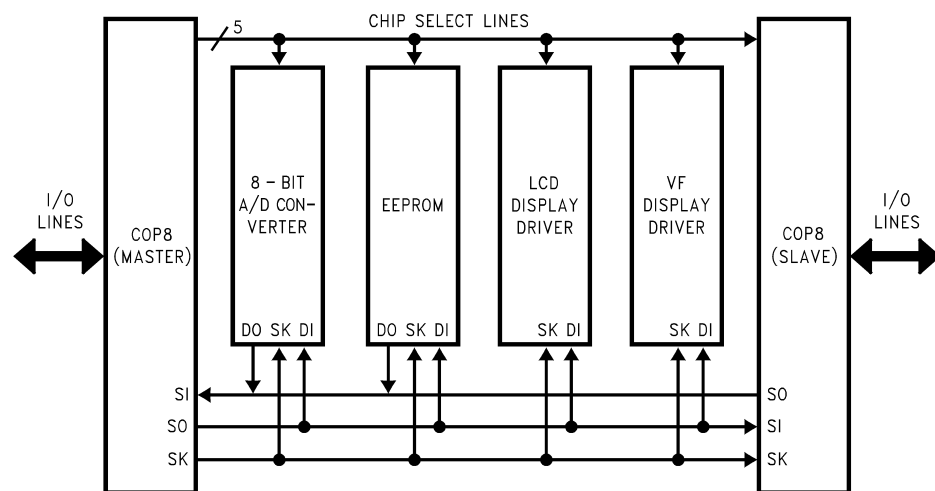
FIGURE 32. MICROWIRE/PLUS Application
