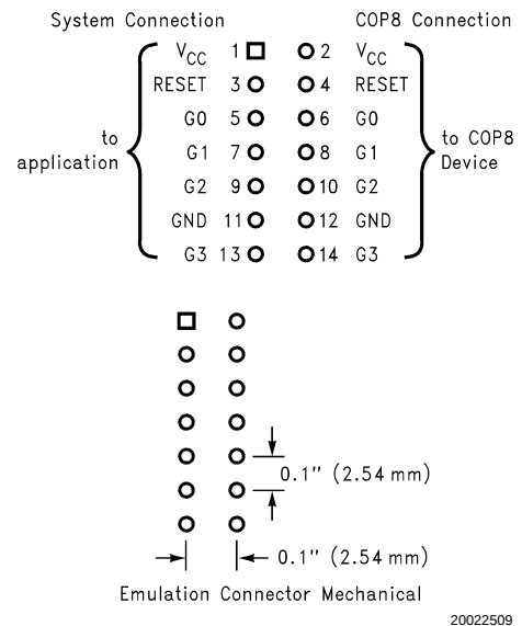
FIGURE 6. Emulation Connection
