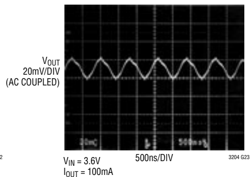
Output Ripple
