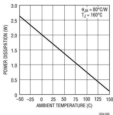
Figure 5. Maximum Power Dissipation vs Ambient Temperature
