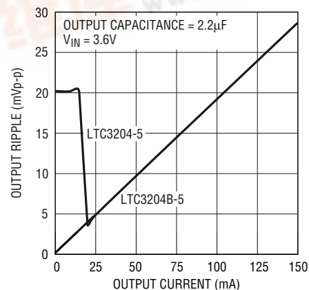
Output Ripple vs Load Current
