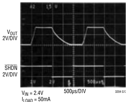
V_{OUT} Soft-Start Response
