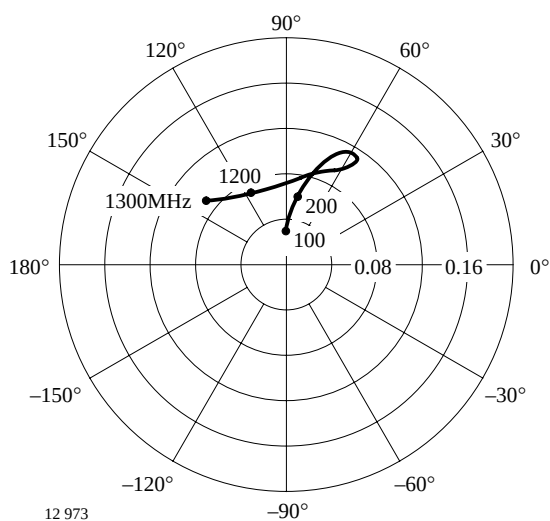
Figure 14. Reverse transmission coefficient
