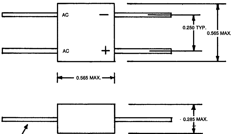
Case Style 2A*
