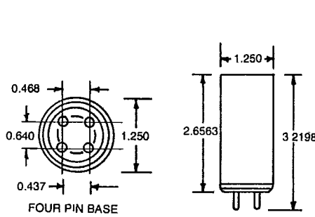
Case Style 6A
