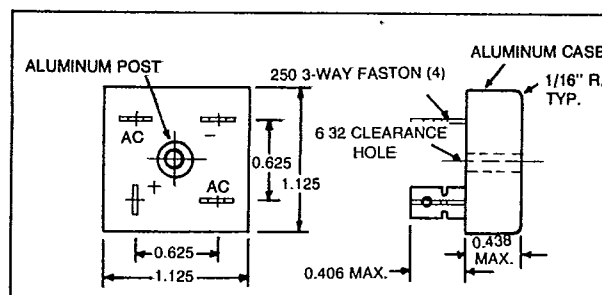
Case Style 3F
