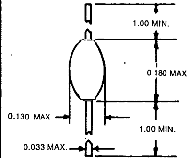
Case Style 1F
