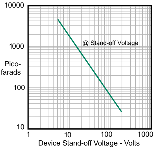
Figure 1 - Capacitance
