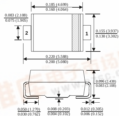
SMB/DO-214AA COLOR BAND DENOTES CATHODE ON UNIDIRECTIONAL DEVICES ONLY. NO COLOR BAND ON BIDIRECTIONAL DEVICES.
