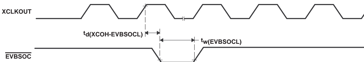
Figure 6–20. EVBSOC Timing
