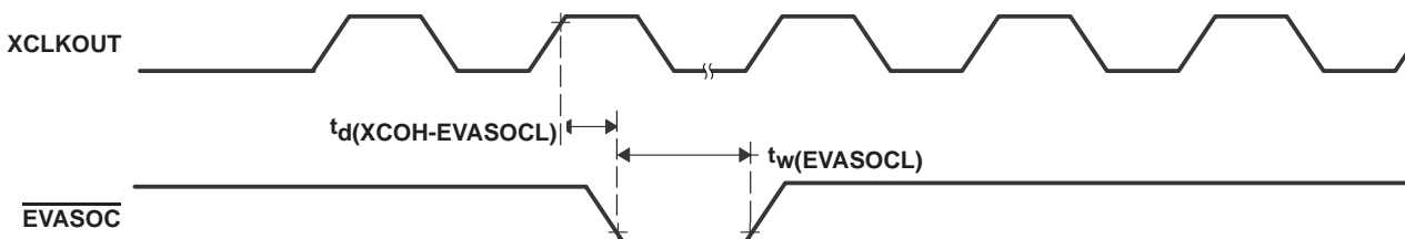
Figure 6–19. EVASOC Timing
