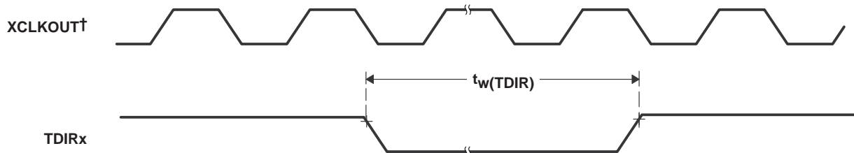
Figure 6–18. TDIRx Timing
