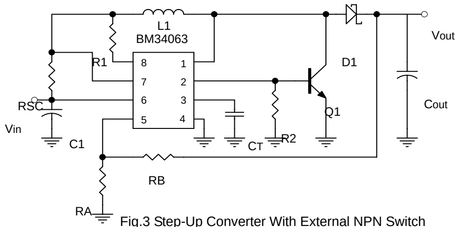
Fig.3 Step-Up Converter With External NPN Switch
