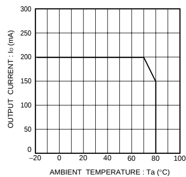
Fig.13 Derating curve
