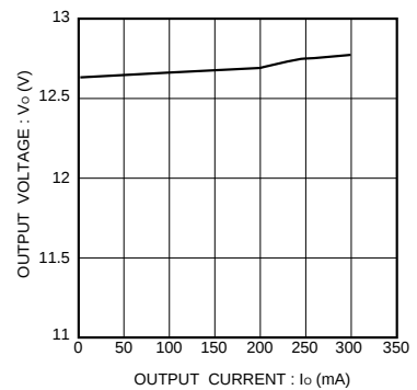
Fig.7 Output characteristic
