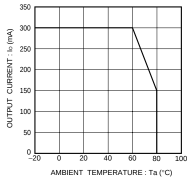
Fig.5 Derating curve
