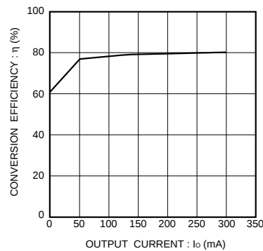
Fig.8 Conversion efficiency
