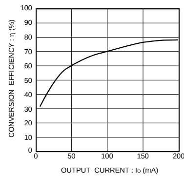
Fig.12 Conversion efficiency
