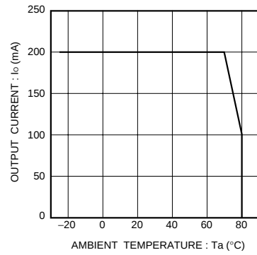
Fig.9 Derating curve
