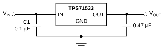
Figure 13. Typical Application Circuit (Fixed Voltage Version)
