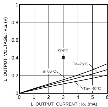
Fig.20 Low output voltage V_{OL}-I_{OL} ( V_{CC}=2.5\text{V} )
