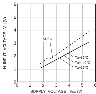
Fig.17 High input voltage V_{IH} (A1,A2,SCL,SDA,WP)
