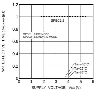
Fig.49 WP high period t_{HIGH:WP}
