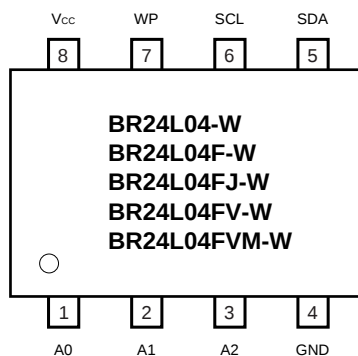
Fig.3 PIN LAYOUT
