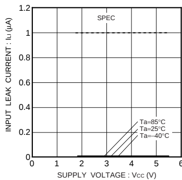
Fig.21 Input leakage current I_I (A1,A2,SCL,WP)
