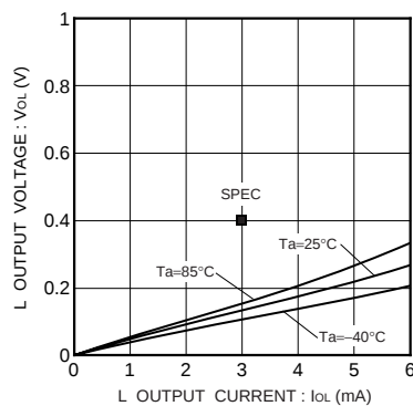
Fig.20 Low output voltage V_{OL} - I_{OL} ( V_{CC} = 2.5V )
