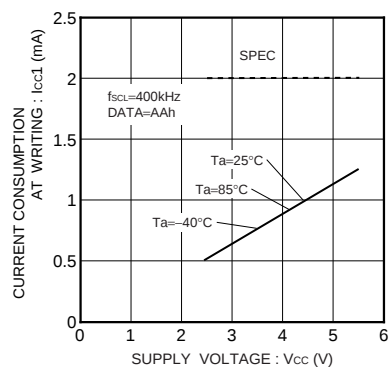
Fig.23 Write operating current I_{CC1} ( f_{SCL} = 400\text{kHz} )
