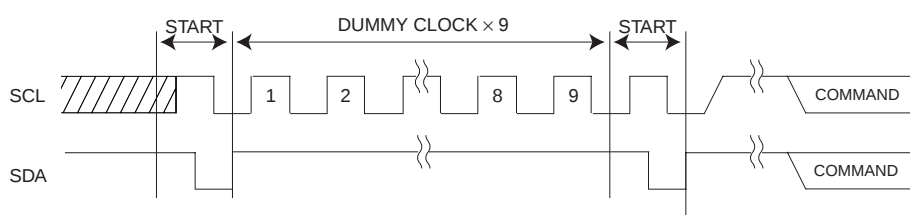
Fig.14-(b) START+ DUMMY CLOCK x 9 + START
