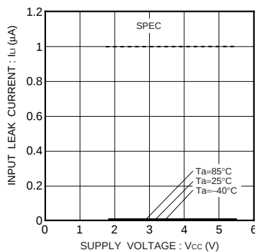
Fig.21 Input leakage current I_I (A2,SCL,WP)
